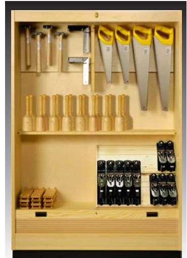
Model 800 64 50 For 24 sets of student's woodwork tools (re. tool schedule).
